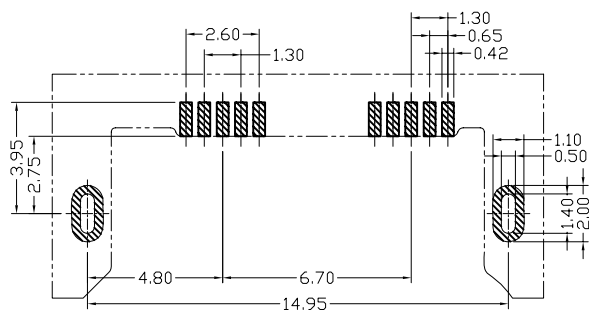
RECOMMEND PCB LAYOUT(TOP VIEW) GENERAL TOLERANCE \pm 0.05
